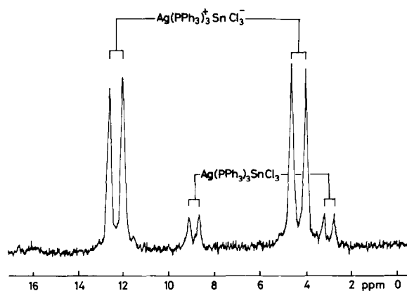
Fig. 1. 31 P NMR spectrum of Ag(PPh 3 ) 3 SnCl 3 in CH 2 Cl 2 at –80 °C.
