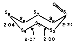
Figure 6. The geometry of \text{S}_8\text{O} .
