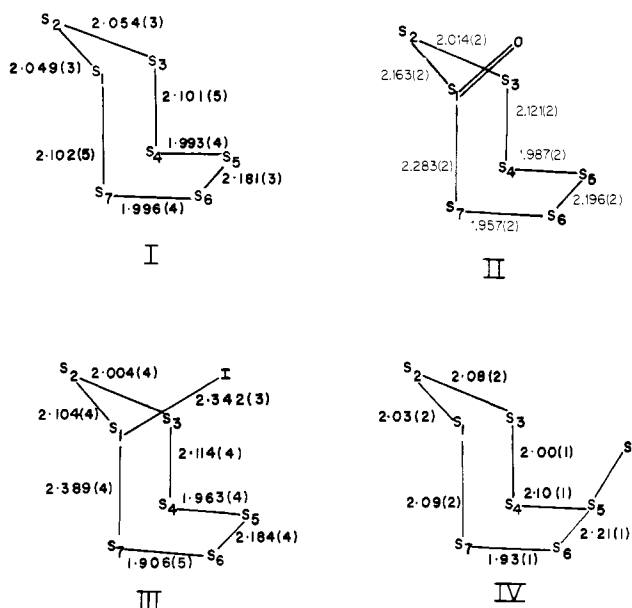
Figure 5. A comparison of the geometries of \delta - \text{S}_7 (I), \text{S}_7\text{O} (II), \text{S}_7\text{I}^+ (III), and the \text{S}_7 chair in \text{S}_{19}^{2+} (IV). The bond distances given for \text{S}_7 are from ref 9a; those given in ref 9b for \delta - \text{S}_7 and \gamma - \text{S}_7 are essentially the same.
