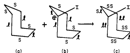
Figure 7. Estimation of bond alternations in \text{S}_7\text{I}^+ : (a) bond alternations due to \text{S}_7 ring; (b) bond alternations due to >\text{S}^+-\text{I} ; (c) resultant. l = long, s = short. The extent of lengthening and shortening decreases with the number of bonds from the source of perturbation.
