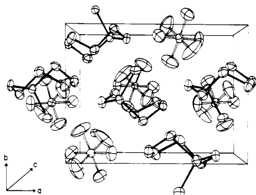
Figure 1. Contents of the S_7ISbF_6 unit cell.
