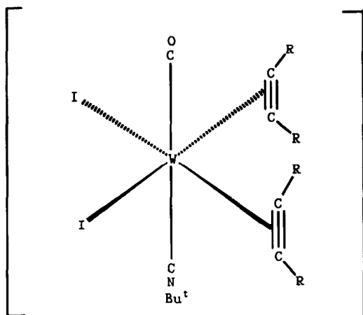
Fig. 1. Proposed structure for [\text{Wl}_2(\text{CO})(\text{CN}^t\text{Bu})(\eta^2\text{-RC}_2\text{R})_2] (1 and 2).
