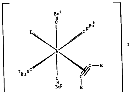
Fig. 4. Proposed structure for [\text{Wl}(\text{CN}^t\text{Bu})_4(\eta^2\text{-RC}_2\text{R})]\text{I} (7 and 8).
