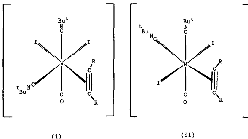
Fig. 2. Possible structures for [\text{Wl}_2(\text{CO})(\text{CN}^t\text{Bu})_2(\eta^2\text{-RC}_2\text{R})] (3 and 4).
