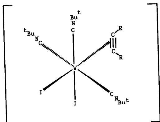
Fig. 3. Most likely structure for [\text{Wl}_2(\text{CN}^t\text{Bu})_3(\eta^2\text{-RC}_2\text{R})] (5 and 6).
