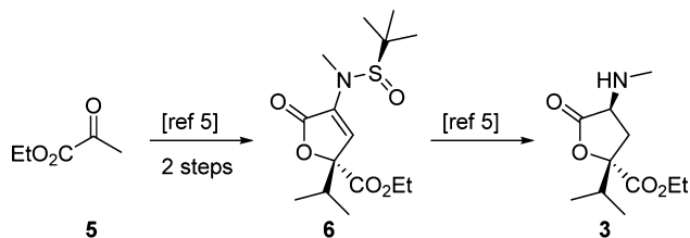
Scheme 2. Synthesis of Masked 4,4-Disubstituted Glutamic Acid Fragment 3 5
