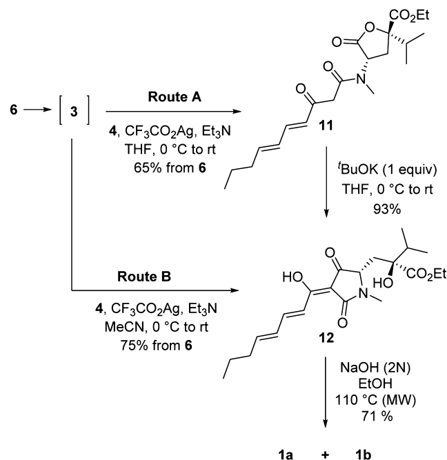
Scheme 4. Total Synthesis of Harzianic Acid ( 1a ) and 5'-Isoharzianic Acid ( 1b )
