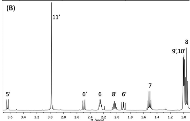
Figure 1. (A) Comparison of selected ^{13}\text{C} NMR signals of isolated harzianic acid ( 1a ) 2 and synthetic 1a and 1b (see Scheme 1 for numbering and Table S1 for a complete comparison of the ^1\text{H} and ^{13}\text{C} NMR spectral data). (a) 400 MHz, \text{CD}_3\text{OD} ; (b) 500 MHz, \text{CD}_3\text{OD} . (B) Section of the ^1\text{H} NMR spectrum of synthetic 1a in \text{CDCl}_3 (see the Supporting Information for the full spectrum).
