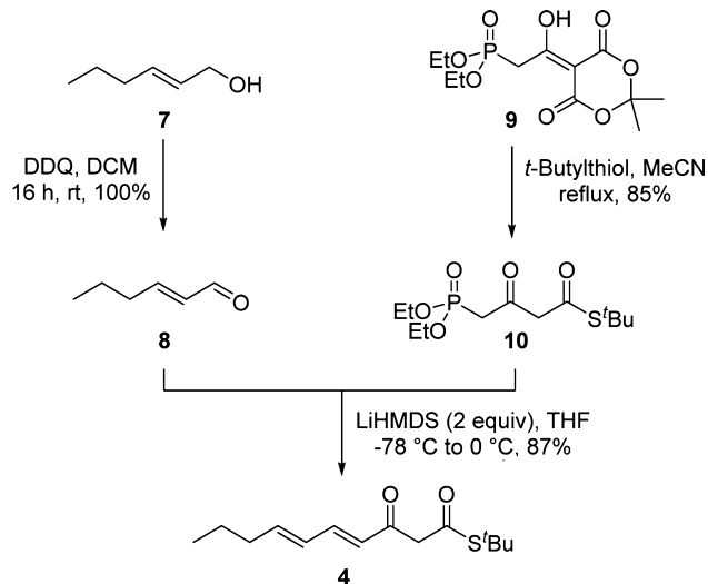
Scheme 3. Synthesis of \beta -Ketothioester Fragment 4
