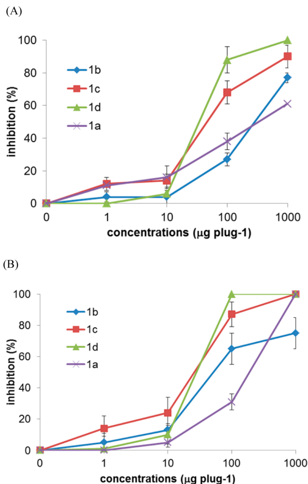
Figure 2. (A) Antibiotic activity of 1a–d against S. rolfii and (B) P. ultimum . Concentrations ranged from 1 to 1000 \mu\text{g plug}^{-1} .
