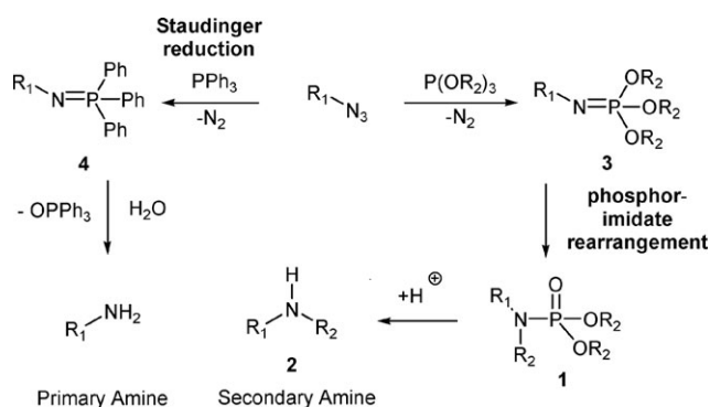
Scheme 1 Synthesis of primary and secondary amines via the Staudinger reduction or the phosphorimide rearrangement.
