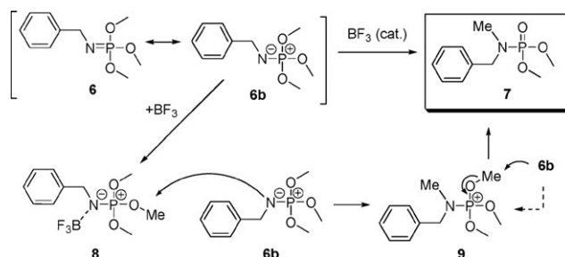
Scheme 2 Mechanism of the \text{BF}_3 \cdot \text{Et}_2\text{O} -catalyzed intermolecular rearrangement of phosphorimide 6 .
