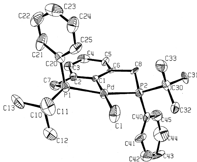
Fig. 1. Thermal ellipsoid (50% probability) drawing of R,R\text{-PdCl}\{\text{C}_6\text{H}_3-2,6-(\text{CH}_2\text{P}^*\text{PhBu}^t)_2\} ( 4 ). Hydrogen atoms have been omitted for clarity.
