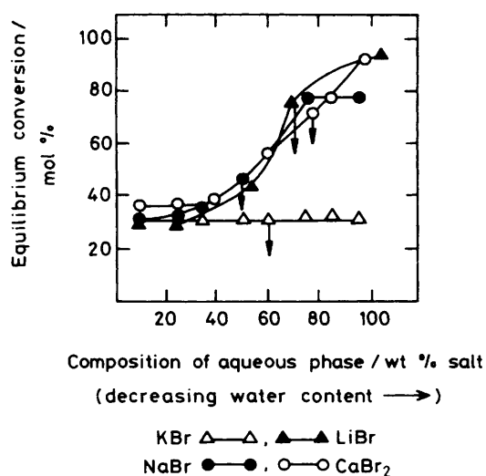
Figure 1. Equilibrium conversion of reaction (3) at 98 °C as a function of the initial aqueous phase composition. With 100% dry salt no reaction is observed at all. The arrows mark the point from which a solid phase is formed during the reaction.
