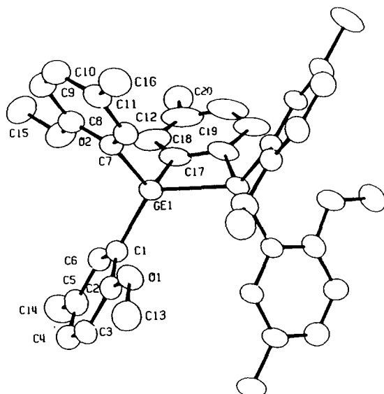
Fig. 4. ORTEP drawing of 9 (note: C(20) is disordered between sites on C(19) and C(19') but has been shown here in a single site for clarity. Please refer to the text for further details).
