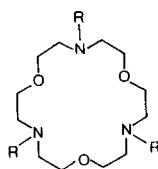
3 R = H 14 R = CH_3
