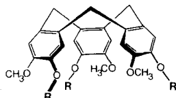
4 R = H 5 R = CH_2COOH 6 R = CH_2COCl 10 R = CH_2CH_2OCH_2COOCH_3 11 R = CH_2CH_2OCH_2COOH 12 R = CH_2CH_2OCH_2COCl
