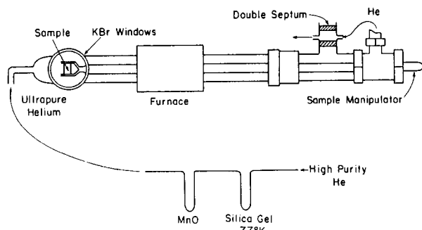
Figure 1. Infrared cell for surface studies.
