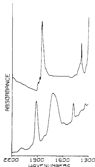
Figure 4. Upper figure: infrared spectrum (Fluorolube mull) of [\text{CpNiCO}]_2 . Lower figure: infrared spectrum of [\text{CpNiCO}]_2 on a DA surface.
