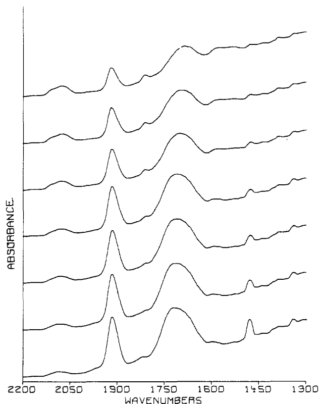
Figure 5. Decomposition of [\text{CpNi(CO)}_2]_2 on a DA surface. The lower tracing was obtained ca. 8 min after deposition of the sample, and the times at which succeeding spectra were obtained (bottom to top) are 11, 13, 16, 27, 35, and 51 min.
