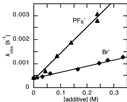
Figure 6. Plots of k_{\text{obs}} vs [\text{additive}] for the oxidative addition of phenyl tosylate to 5. Additives: \text{NBu}_4\text{PF}_6 (triangles) and \text{NBu}_4\text{Br} (diamonds).
