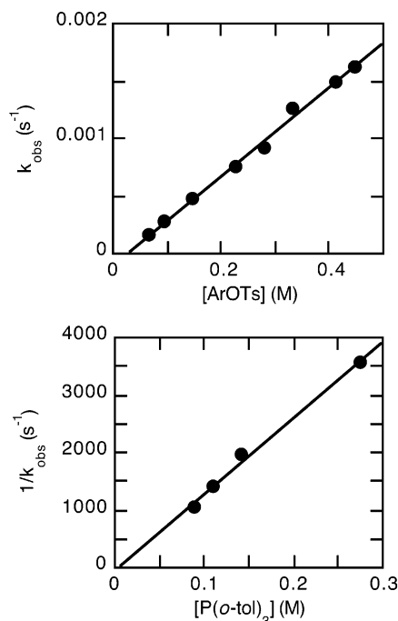
Figure 5. Plots of k_{\text{obs}} vs [\text{PhOTs}] and 1/k_{\text{obs}} vs [\text{P}(\text{o-tol})_3] for the oxidative addition of phenyl tosylate to complex 5.
