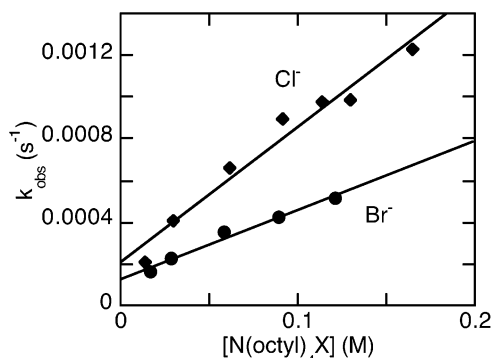
Figure 4. Plots of k_{\text{obs}} vs [\text{N(octyl)}_4\text{Br}] (circles) and k_{\text{obs}} vs [\text{N(octyl)}_4\text{Cl}] (diamonds) for the oxidative addition of ArOTf to \text{Pd}[\text{P(o-tolyl)}_3]_2 in benzene- d_6 solvent in the presence of added halide.
