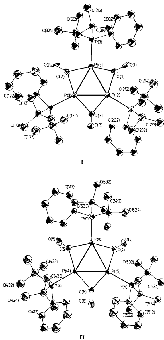
Fig. 1. ORTEP diagrams of the two independent molecules of 1c with hydrogen atoms omitted. The thermal ellipsoids are represented by 30% probability contours.
