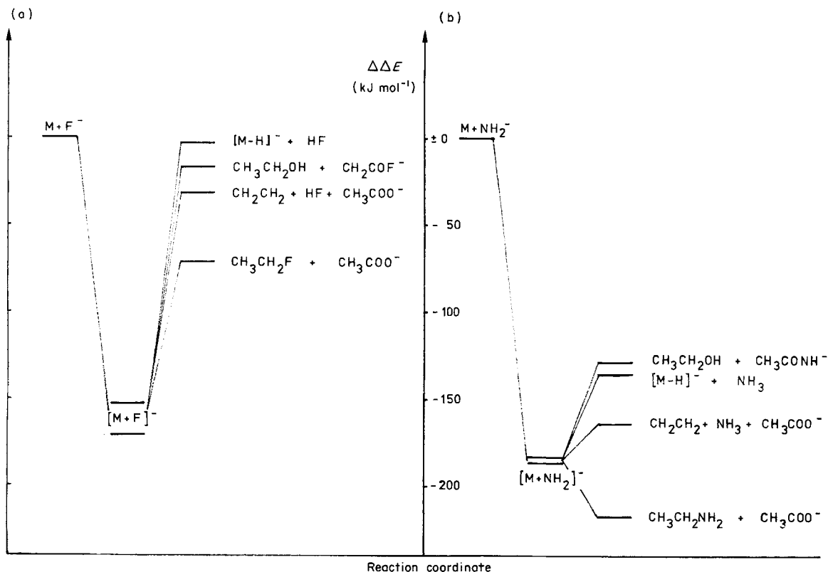
Figure 3. Schematic reaction energy diagram of reactions (7a) and (7b) calculated by MINDO/3.
