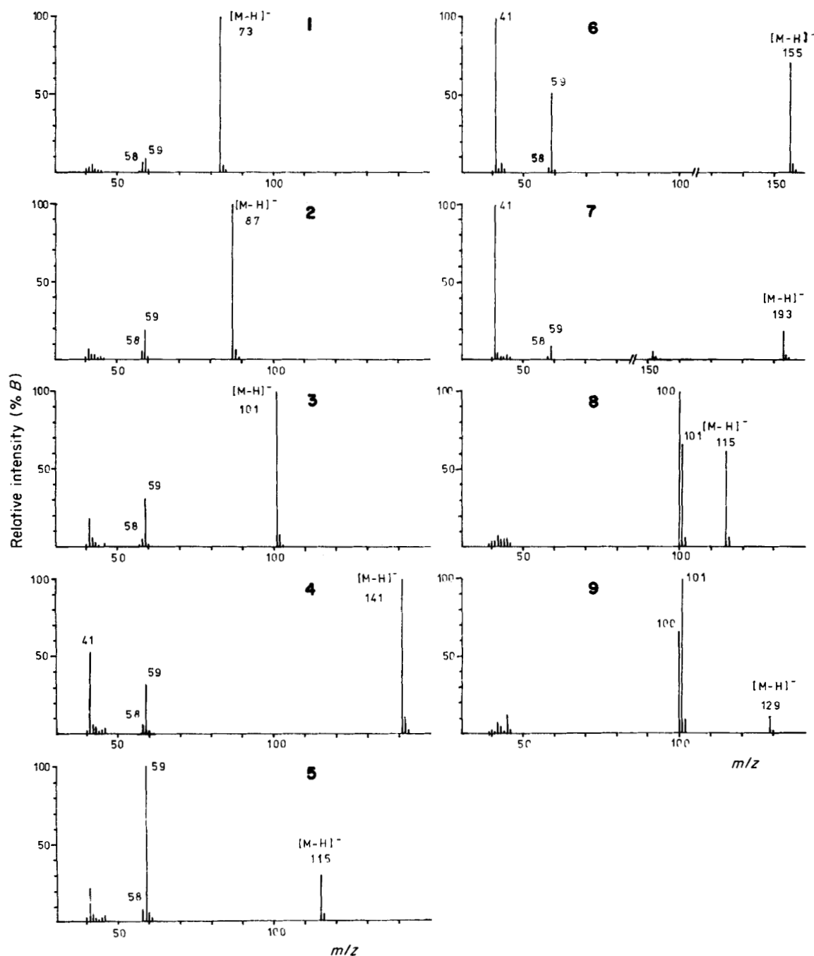
Figure 2. NCI(NH 2 - ) mass spectra of the acetates 1-5 and 7 and the trimethylacetates 8 and 9.
