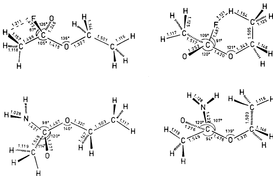
Figure 4. Geometries of the stable conformations of the tetrahedral addition complexes of reactions (7a) and (7b) calculated by MINDO/3.
