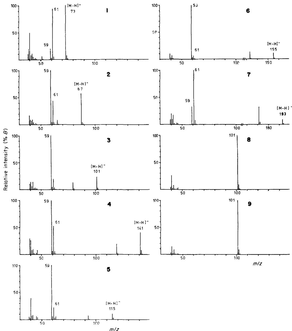
Figure 1. NCI( F^- ) mass spectra of the acetates 1-7 and the trimethylacetates 8 and 9 .
