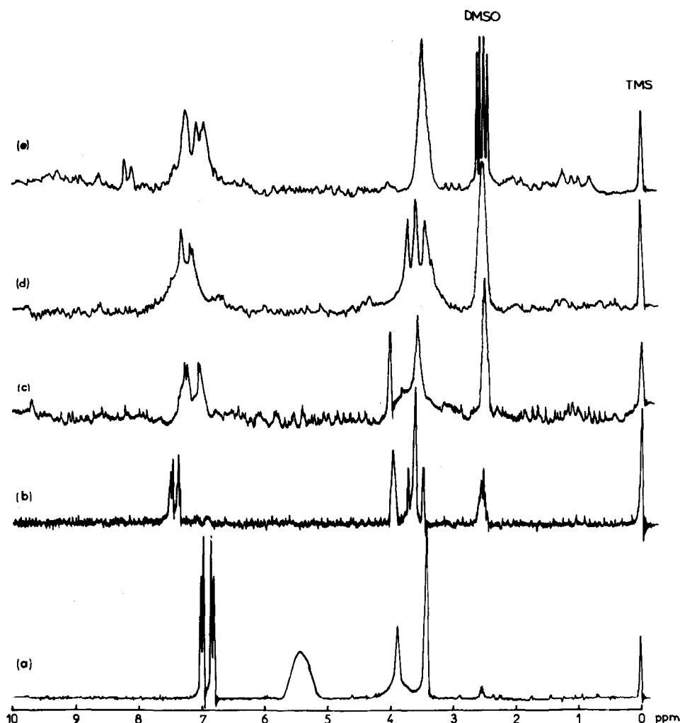
Figure 2. ^1\text{H} n.m.r. spectra in \text{DMSO}-d_7 solution of: (a) SHmi, (b) \text{Pt}(\text{SHmi})_2\text{Cl}_2 , (c) \text{Pd}(\text{SHmi})_2\text{Cl}_2 , (d) \text{Pt}(\text{Smi})_2 , (e) \text{Pd}(\text{Smi})_2 .
