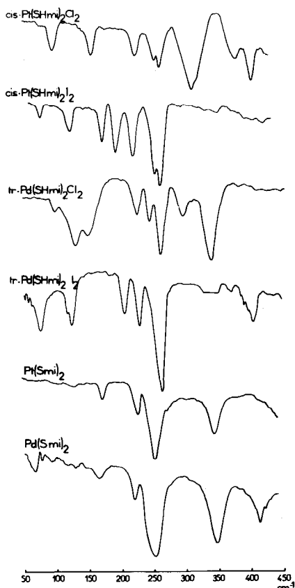
Figure 1. Far infrared spectra (450–50 cm -1 ) of cis -Pt and trans -Pd complexes with 2-mercapto,1-methylimidazole (SHmi).
