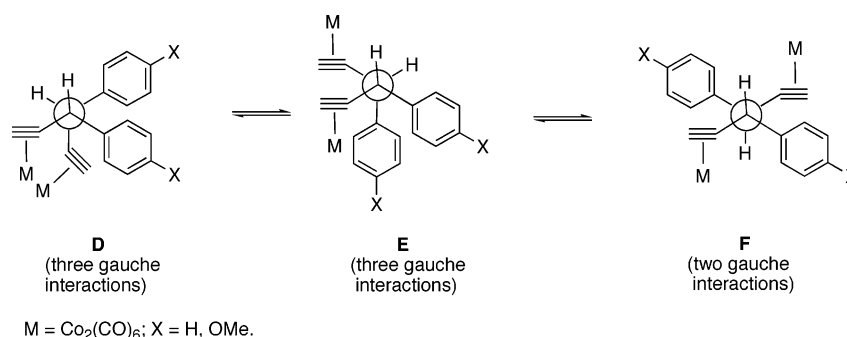
Figure 3. Formation of meso -diastereomers 7–9: staggered orientations of converging propargyl radicals.
