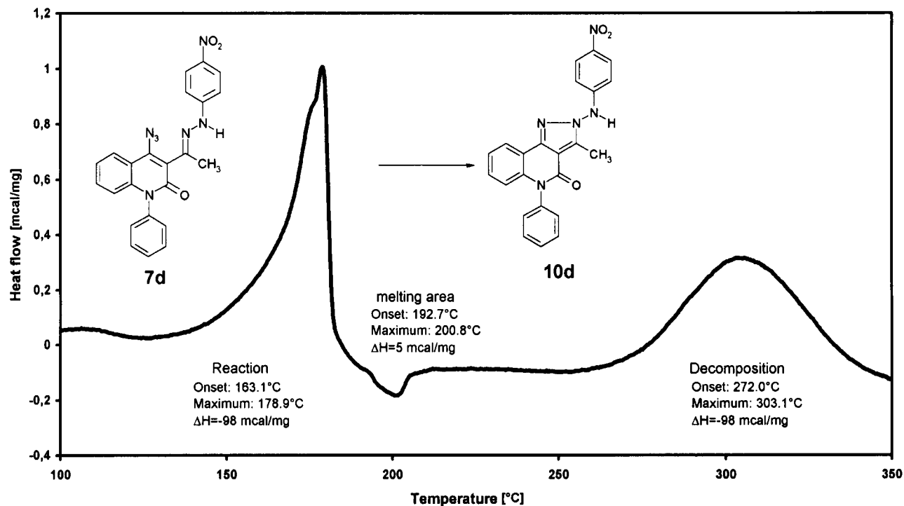
Figure 1. Differential scanning calorimetry diagram of 4-azido-3-[1-(4-nitrophenylhydrazonoethyl)-2(1 H )-quinolone ( 7d ).
