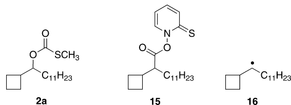
Figure 5. Xanthate 2a and PTOC 15 precursors of substituted cyclobutylcarbinyl radical probe 16 .
