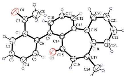
Fig. 1 Single crystal structure of 3a .
