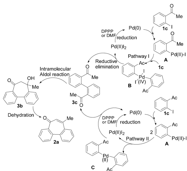
Fig. 2 The proposed reaction mechanism.
