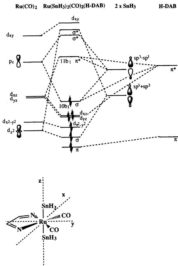
Figure 6. Qualitative MO scheme of Ru(SnH 3 ) 2 (CO) 2 (H-DAB) and chosen orientation of the axes.
