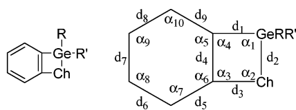
Figure 5. Theoretically optimized structure of 3 at the B3LYP/6-31G(d) level.
