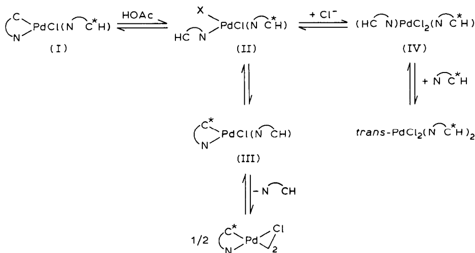
SCHEME 1
