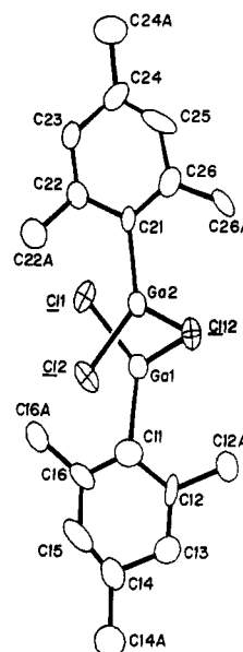
Figure 2. The crystallographic asymmetric unit of dichloromesitylgallium(III) with atomic labeling. The view is perpendicular to that of Figure 1, and the structure extends by Ga(2) linking to a further symmetry-related bridging chloride ligand above the position of Cl(12) and by Ga(1) linking to a further bridging chloride ligand below the position of Cl(12).
