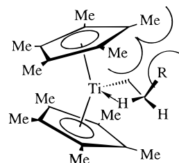
Figure 11. Steric congestion in a \beta -agostic alkyl complex of \text{Cp}^*_2\text{Ti} .
