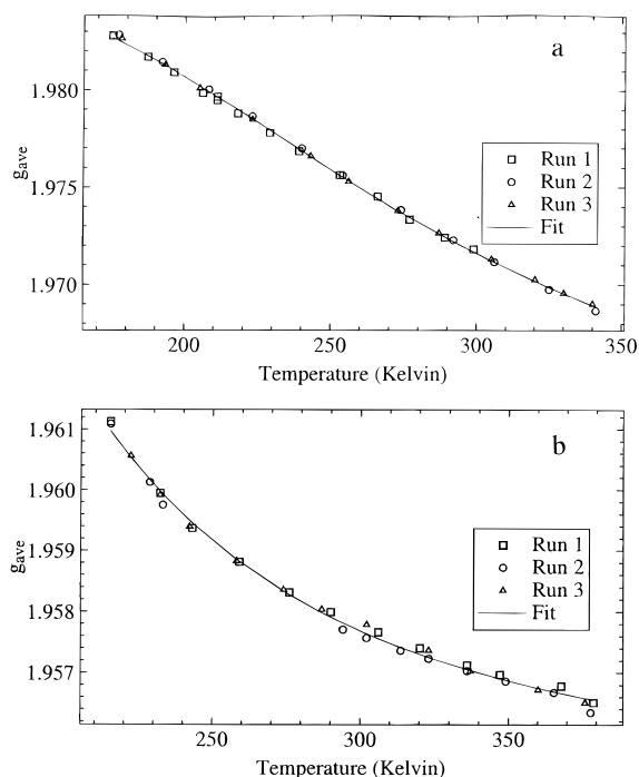
Figure 10. Observed g_{\text{ave}} versus temperature for \text{Cp}^*_2\text{TiEt} (a) and \text{Cp}^*_2\text{TiN}(\text{Me})\text{Ph} (b). The different symbols are for independent data runs, and the line is a least-squares fit to eq 4.
