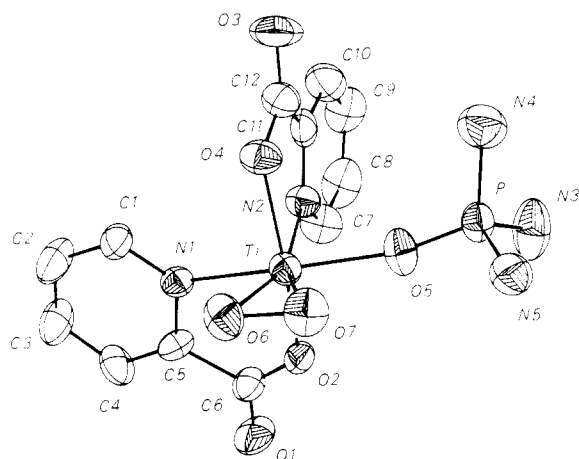
Figure 1. Molecular structure of \text{Ti}(\text{O}_2)(\text{C}_6\text{H}_4\text{NO}_2)_2 \cdot \text{OPN}_3\text{C}_6\text{H}_{18} (1).
