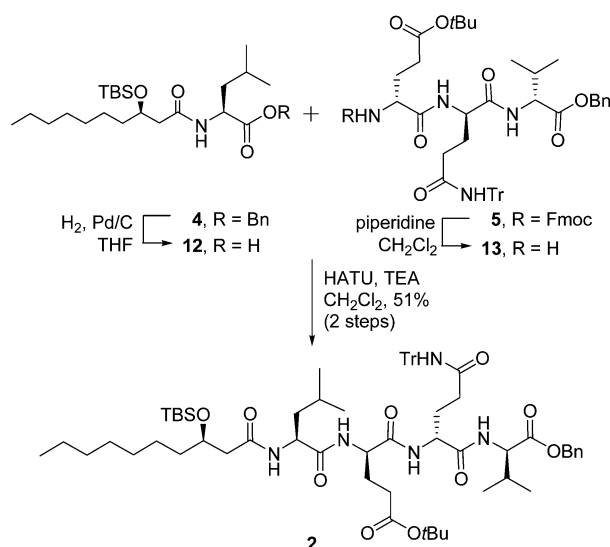
Scheme 5. Synthesis of Side Chain 2
