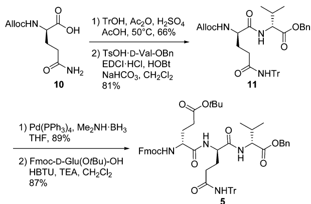
Scheme 4. Preparation of Tripeptide 5
