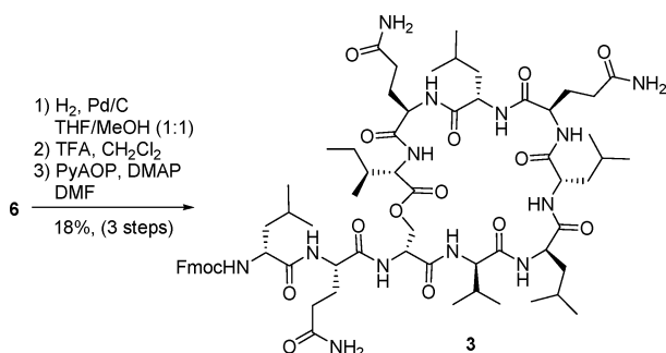
Scheme 8. Synthesis of Cyclodepsipeptide 3
