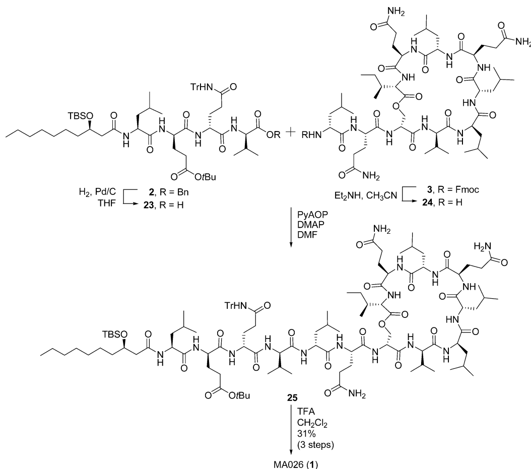
Scheme 9. Synthesis of MA026 (1)
