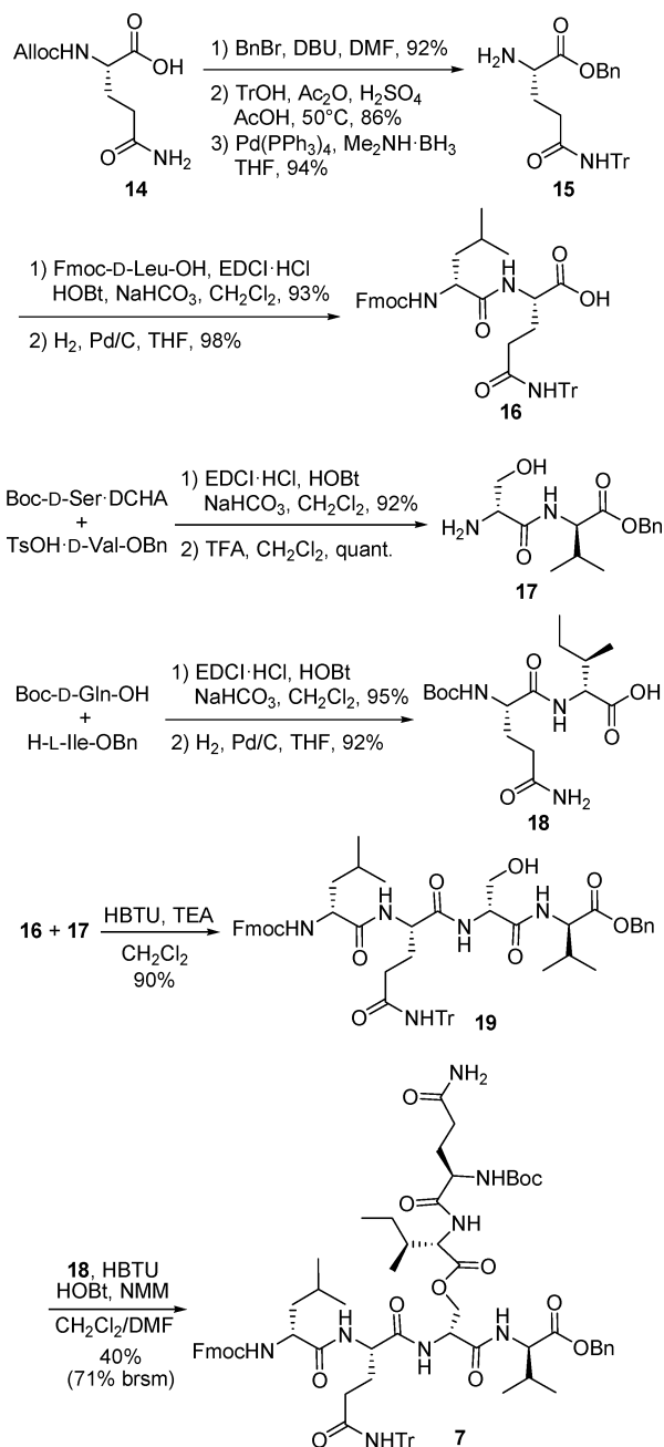
Scheme 6. Construction of Hexadepsipeptide 7
