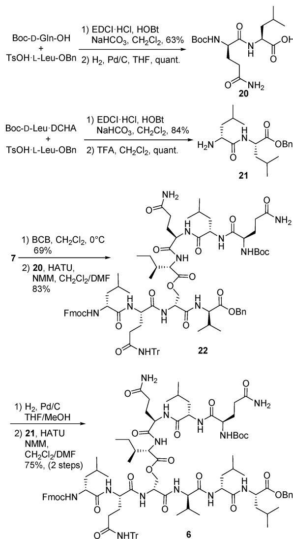
Scheme 7. Synthesis of Decadepsipeptide 6
