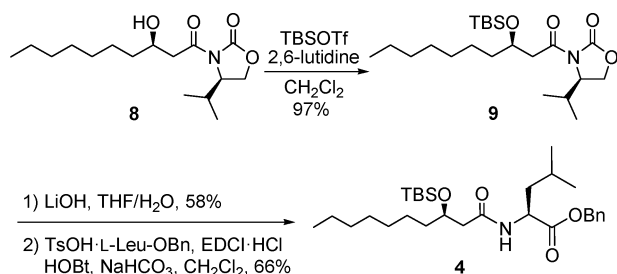
Scheme 3. Synthesis of Fatty Acid Moiety 4
