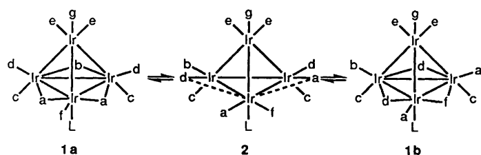
Scheme 1 Modified Cotton mechanism for carbonyl scrambling in [\text{Ir}_4(\text{CO})_{11}L] . The lower-case letters refer to carbonyl ligands
