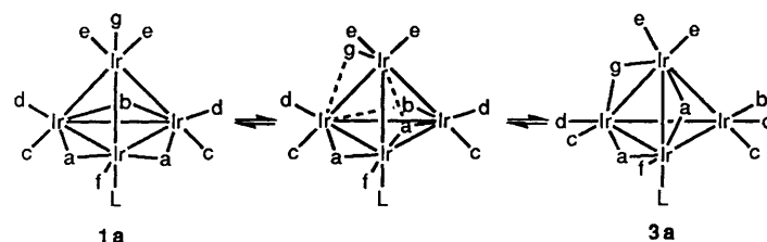
Scheme 2 Face-bridged mechanism for carbonyl scrambling in [\text{Ir}_4(\text{CO})_{11}L] derivatives
