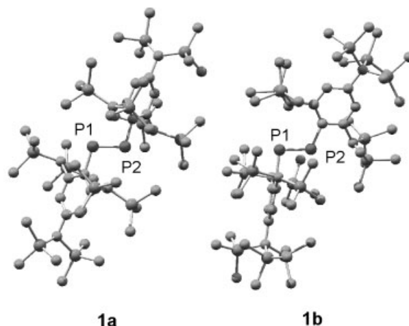
Figure 3. Side views of the diphosphenes 1a and 1b
