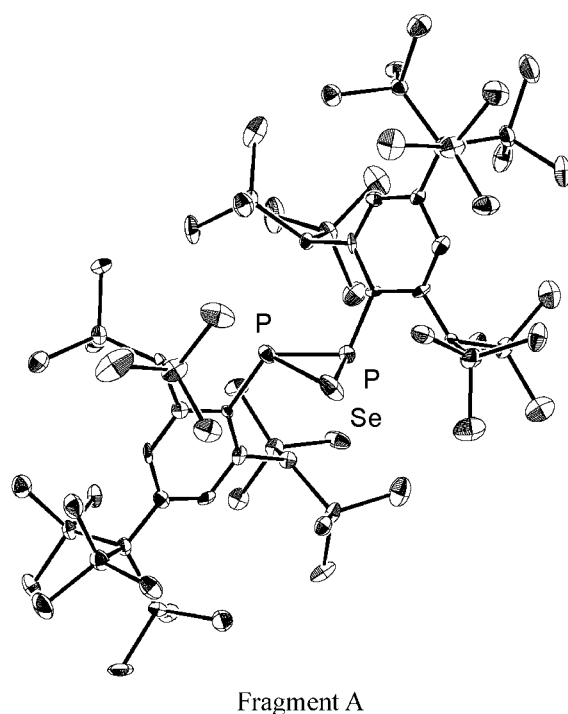
Figure 7. ORTEP drawing of selenadiphosphirane 21 with thermal ellipsoid plot (50% probability). The fragment of solvated hexane was omitted for clarity
