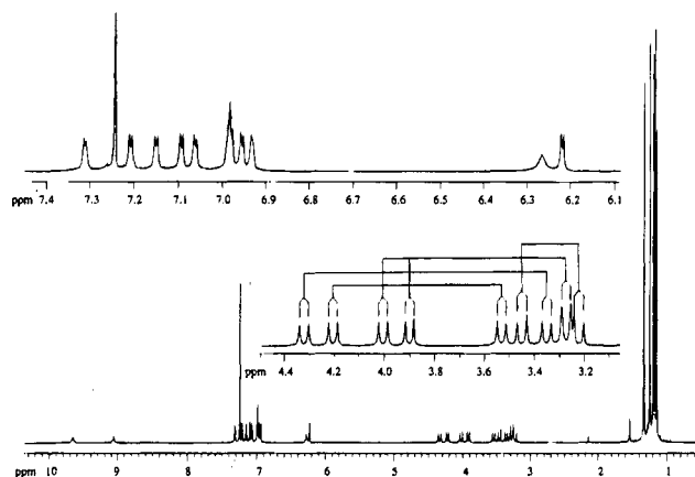
Figure 1. ^1\text{H} NMR spectrum (400 MHz, \text{CDCl}_3 ) of 4b .
