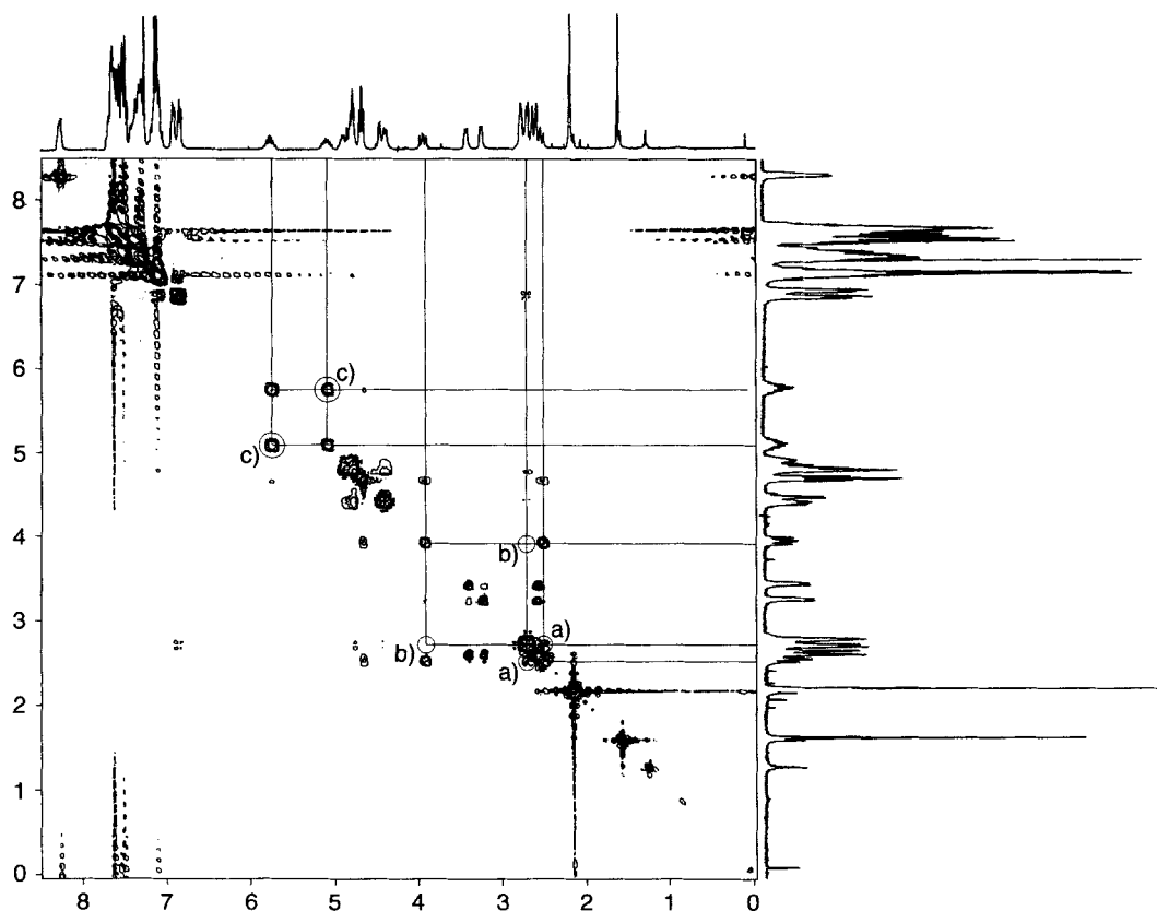
Fig. 6. Homonuclear ^1\text{H} -NOESY spectrum of 4 . Cross-peaks (○): a) NOE between \text{H}_f\text{-C}(300) of the major isomer and the methylene proton of the benzyl substituent \text{H-C}(400) . b) No cross-peak between \text{H}_f\text{-C}(300) of the minor isomer and \text{H-C}(400) . c) Exchange cross-peaks between the central allyl protons ( \text{H-C}(200) ) of the two isomers.
