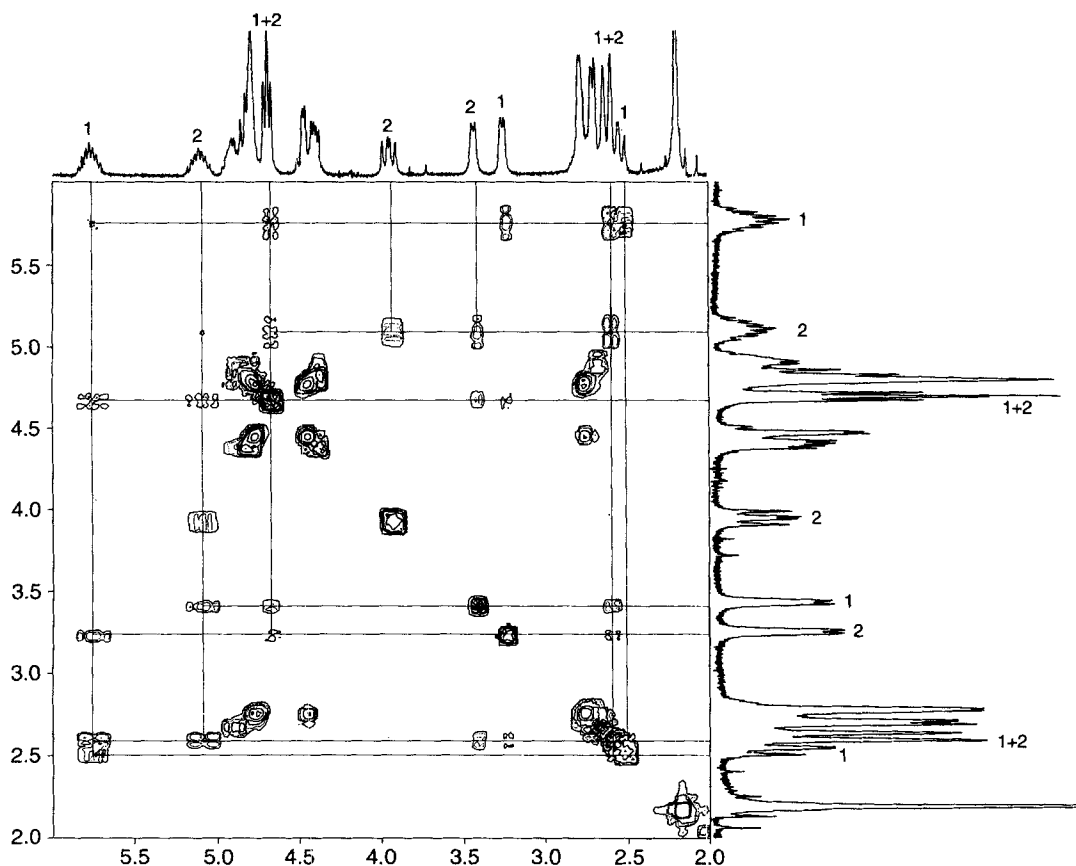
Fig. 5. Homonuclear ^1\text{H} -COSY spectrum of 4 . 1: 'endo' isomer; 2: 'exo' isomer.
