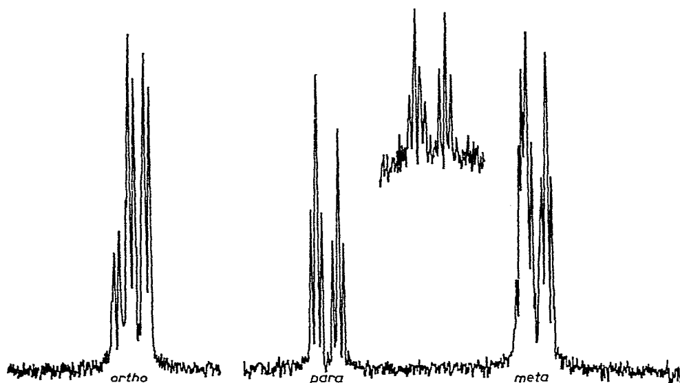
Fig. 2. The ^{19}\text{F} NMR spectrum of pentafluorophenylthioiron tricarbonyl dimer. The sample was dissolved in \text{CFCl}_3 as the internal standard. The insert shows the para region of the spectrum when the sample is dissolved in benzene. Shifts, relative to \text{CFCl}_3 , were: large ortho doublet centred at 125 ppm; large para doublet centred at 151.6 ppm and a meta doublet centred at 160.8 ppm.
