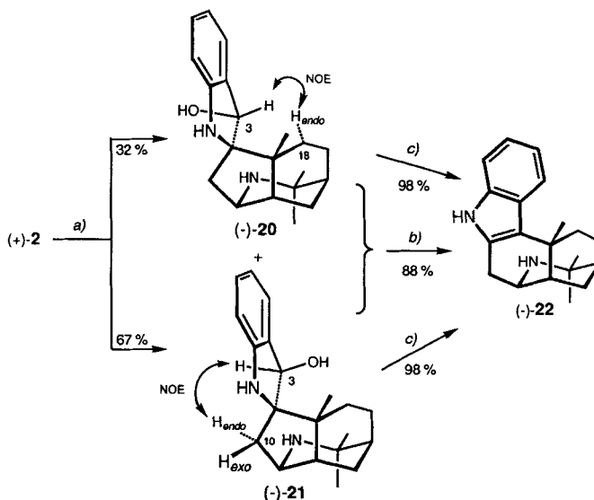
Scheme 6 a)
