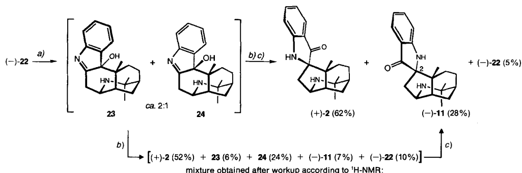
Scheme 7
