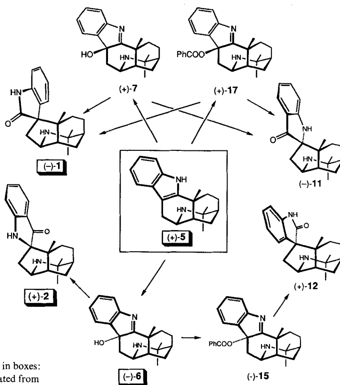
Scheme 8
