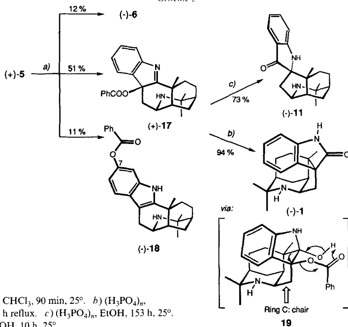
Scheme 5
