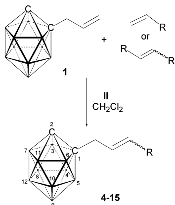
Scheme 1. Cross Metathesis Reactions of 1-(CH 2 =CHCH 2 )-1,2-C 2 B 10 H 11 (1) with Functional Olefins Catalyzed by II
