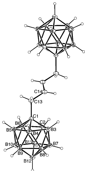
Figure 2. ORTEP representation of the structure of 1,1'-(CH 2 =CHCH 2 )-(1,2-C 2 B 10 H 11 ) 2 ( 3 ). Selected bond distances (Å) and angles (deg): C1–C2, 1.648(2); C1–B3, 1.724(2); C1–B4, 1.705(2); C1–B5, 1.706(2); C1–B6, 1.727(2); C1–C13, 1.528(2); C13–C14, 1.496(2); C14–C14*, 1.321(4); C13–C1–C2, 120.14(9); C13–C1–B3, 118.00(10); C13–C1–B4, 120.68(9); C13–C1–B5, 119.93(10); C13–C1–B6, 116.67(9); C1–C13–C14, 114.65(11); C13–C14–C14*, 123.3(3).
