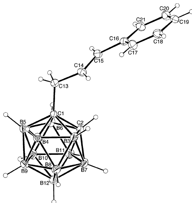
Figure 3. ORTEP representation of the structure of 1-(C 6 H 5 CH=CHCH 2 )-1,2-C 2 B 10 H 11 (5). Selected bond distances (Å) and angles (deg): C1–C2, 1.645(2); C1–B3, 1.729(2); C1–B4, 1.703(2); C1–B5, 1.710(2); C1–B6, 1.733(2); C1–C13, 1.529(2); C13–C14, 1.494(3); C14–C15, 1.323(3); C15–C16, 1.488(2); C13–C1–C2, 119.69(12); C13–C1–B3, 119.26(13); C13–C1–B4, 122.07(13); C13–C1–B5, 119.55(12); C13–C1–B6, 115.62(14); C1–C13–C14, 116.7(2); C13–C14–C15, 124.9(2); C14–C15–C16, 126.7(2); C15–C16–C17, 120.81(14); C15–C16–C21, 119.14(14).
