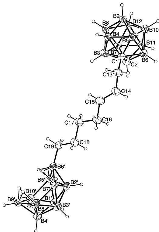
Figure 6. ORTEP representation of the structure of 1-[1-(1,2-C 2 B 10 H 11 )]-CH 2 CH=CH(CH 2 ) 4 -7-(6-B 10 H 13 ) ( 30 ). Selected bond distances (Å) and angles (deg): C1–C2, 1.640(5); C1–B3, 1.741(7); C1–B4, 1.712(5); C1–B5, 1.703(6); C1–B6, 1.701(6); C1–C13, 1.529(5); C13–C14, 1.464(6); C14–C15, 1.333(6); C15–C16, 1.473(6); C16–C17, 1.535(6); C17–C18, 1.519(6); C18–C19, 1.527(6); C19–B6', 1.571(6); B2'–B6', 1.742(6); B5'–B6', 1.795(7); B6'–B7', 1.813(6); B8'–B9', 1.770(7); B4'–B9', 1.726(7); B9'–B10', 1.787(8); C13–C1–C2, 120.8(3); C13–C1–B3, 117.5(4); C13–C1–B4, 119.5(3); C13–C1–B5, 119.4(3); C13–C1–B6, 117.7(4); C1–C13–C14, 115.6(4); C13–C14–C15, 121.1(4); C14–C15–C16, 125.6(5); C15–C16–C17, 112.4(4); C16–C17–C18, 110.3(4); C17–C18–C19, 113.8(4); C18–C19–B6', 114.4(4).
