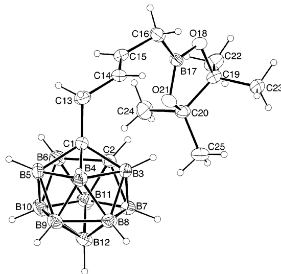
Figure 5. ORTEP representation of 1-[(CH 3 ) 4 C 2 O 2 ]BCH 2 CH=CHCH 2 -1,2- C_2B_{10}H_{11} ( 15 ). Selected bond distances (Å) and angles (deg): C1–C2, 1.650(4); C1–B3, 1.716(4); C1–B4, 1.701(4); C1–B5, 1.707(4); C1–B6, 1.725(4); C1–C13, 1.533(3); C13–C14, 1.482(3); C14–C15, 1.324(4); C15–C16, 1.487(4); C16–B17, 1.572(4); B17–O18, 1.360(3); B17–O21, 1.370(3); O18–C19, 1.464(3); C19–C20, 1.566(4); C20–O21, 1.461(3); C19–C22, 1.520(4); C19–C23, 1.514(4); C20–C24, 1.522(4); C20–C25, 1.516(4); C13–C1–C2, 118.9(2); C13–C1–B3, 117.2(2); C13–C1–B4, 121.2(2); C13–C1–B5, 121.0(2); C13–C1–B6, 116.9(2); C1–C13–C14, 115.3(2); C13–C14–C15, 124.7(3); C14–C15–C16, 127.1(4); C15–C16–B17, 118.2(2); C16–B17–O18, 124.2(2); C16–B17–O21, 122.2(2); O18–B17–O21, 113.5(2); B17–O18–C19, 107.8(2); O18–C19–C20, 102.0(2); C19–C20–O21, 102.6(2); C22–C19–C23, 110.0(2); C24–C20–C25, 110.8(2).
