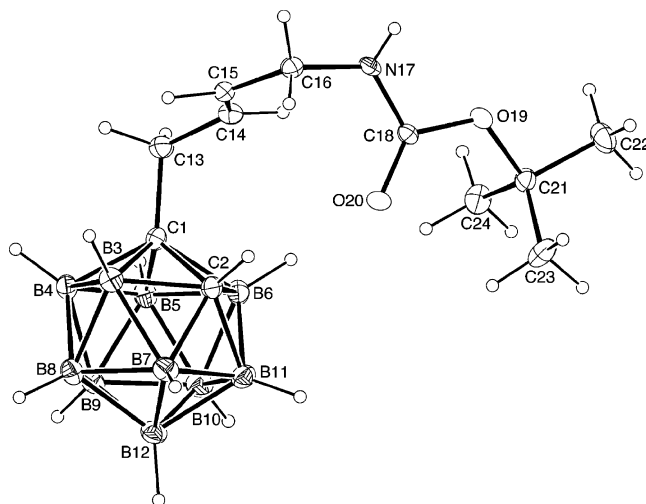
Figure 4. ORTEP representation of the structure of 1-[ t -C 4 H 9 OC(O)NHCH 2 CH=CHCH 2 ]-1,2-C 2 B 10 H 11 (13). Selected bond distances (Å) and angles (deg): C1–C2, 1.658(3); C1–B3, 1.722(3); C1–B4, 1.713(3); C1–B5, 1.712(3); C1–B6, 1.726(3); C1–C13, 1.514(3); C13–C14, 1.501(3); C14–C15, 1.322(3); C15–C16, 1.504(3); C16–N17, 1.448(3); N17–C18, 1.341(3); C18–O19, 1.347(2); C18–O20, 1.223(3); O19–C21, 1.482(2); C21–C22, 1.522(3); C21–C23, 1.518(3); C21–C24, 1.517(3); C13–C1–C2, 118.8(2); C13–C1–B3, 116.7(2); C13–C1–B4, 121.2(2); C13–C1–B5, 121.7(2); C13–C1–B6, 117.4(2); C1–C13–C14, 113.6(2); C13–C14–C15, 122.3(2); C14–C15–C16, 126.1(2); C15–C16–N17, 115.0(2); C16–N17–C18, 121.6(2); O19–C18–O20, 125.2(2); C18–O19–C21, 119.7(2); O19–C21–C22, 102.4(2); O19–C21–C23, 111.5(2); O19–C21–C24, 108.6(2).
