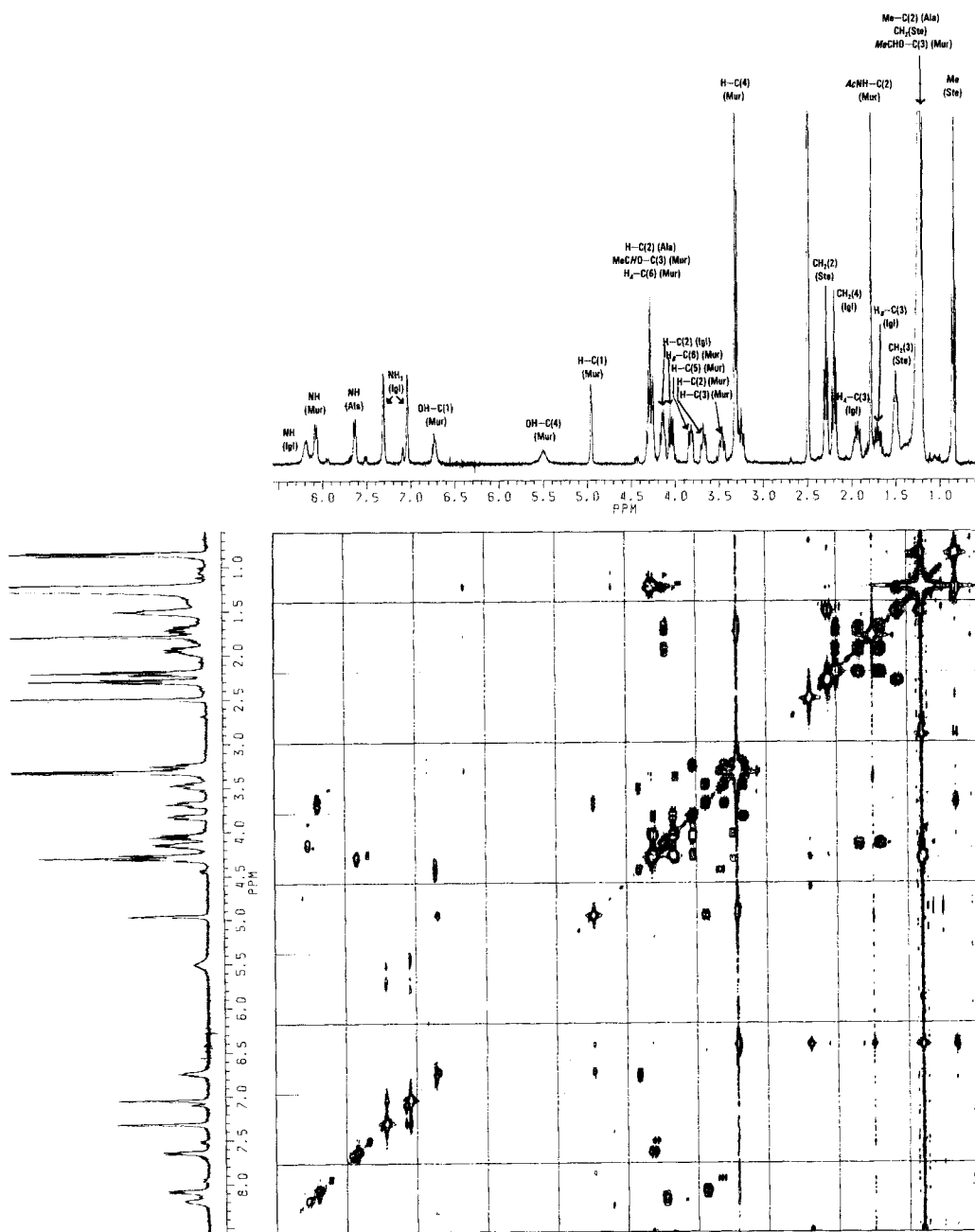
Figure. 2D-COSY(90) of 1 in D_6 DMSO at 360 MHz. Assignments given only for the major \alpha -D-isomer.
