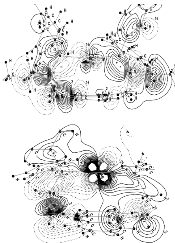
Figure 3. Contour plots of HF/LanL2DZ molecular orbital 159 (upper), which indicates tri-center Ag–CN bonding in L1Ag + , and 117 (lower) in L2Ag + (for reference) on the plane roughly containing the neighboring N–P–Ag–P–N and C–P–Ag–P–C atoms, respectively. Solid contours are at 0.005, 0.010, ..., 0.095 e/a_0^3 , and negative contours are dashed.
