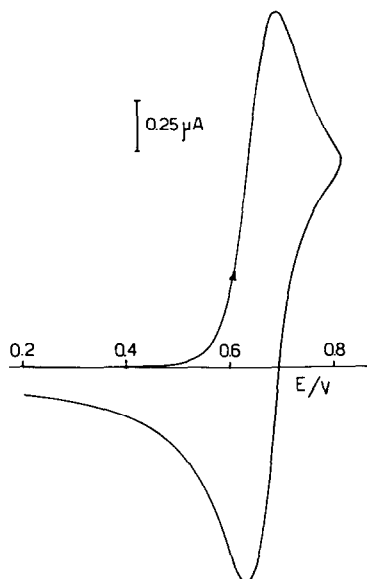
Fig. 2. Cyclic voltammogram for oxydation of 3.1 \times 10^{-3} M [\text{Fe}(\eta^5\text{-C}_5\text{H}_4\text{PPh}_2)_2\text{PtCl}_2] in 1,2-dichloroethane containing (n\text{-Bu}_4\text{N})\text{ClO}_4 at 25^\circ\text{C} (Pt microelectrode, \text{Ag}/0.1\text{ M AgClO}_4 in \text{CH}_3\text{CN} as reference electrode). Scan rate 150\text{ mV s}^{-1} .
