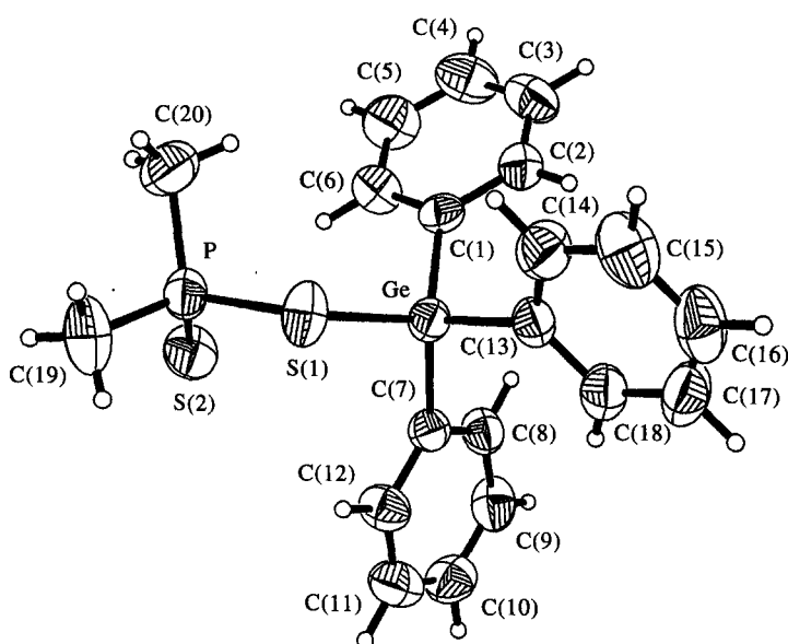
Fig. 1. ORTEP-like view of the \text{Ph}_3\text{GeS}(\text{S})\text{PMe}_2 (1) molecule.
