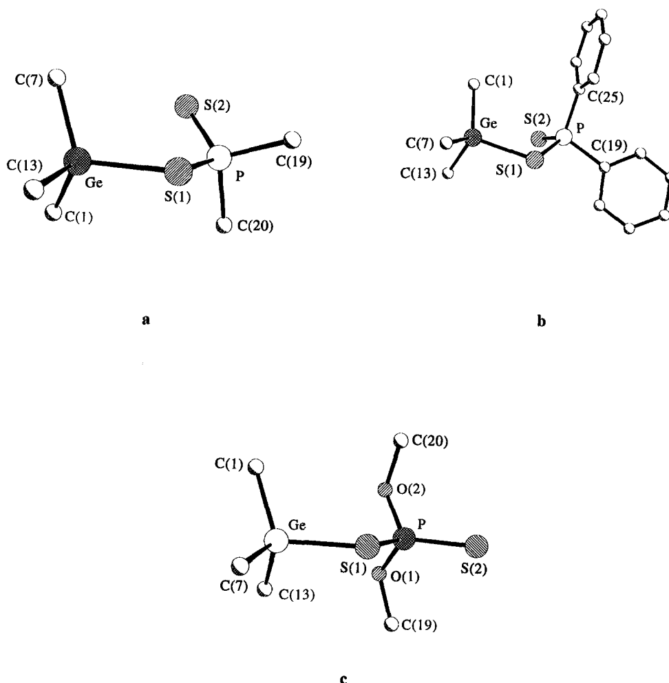
Fig. 3. Comparative orientation of the 1,1-dithiophosphorus ligand in: (a) \text{Ph}_3\text{GeS}(\text{S})\text{PMe}_2 ; (b) \text{Ph}_3\text{GeS}(\text{S})\text{PPh}_2 (this work); and (c) \text{Ph}_3\text{GeS}(\text{S})\text{P}(\text{OMe})_2 (redrawn from the atomic coordinates given in ref. 2). Only ipso -carbons of the phenyl groups attached to germanium are shown, the others being omitted for clarity.
