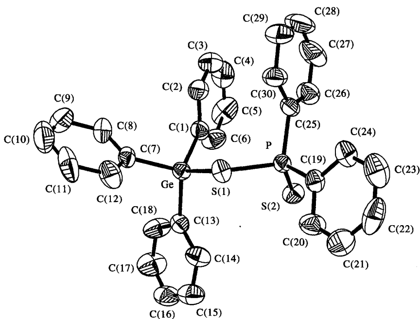
Fig. 2. ORTEP-like view of the \text{Ph}_3\text{GeS}(\text{S})\text{PPh}_2 (3) molecule.
