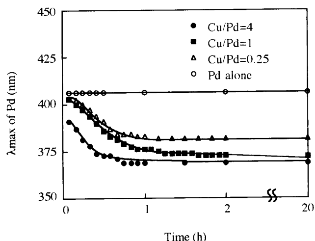
Fig. 4. Time course of the shift of the \lambda_{\max} of \text{Pd}(\text{OAc})_2 in TFA. Conditions: total amount of \text{Pd}(\text{OAc})_2 and \text{Cu}(\text{OAc})_2 0.05 mmol, TFA 10 ml, rt.
