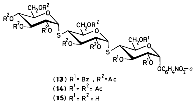
benzoate ( 10 ) by the action of sodium methylate in methanol, followed by a direct attempt at displacement of the C-4 triflate in the o -nitrophenyl \alpha -D-galactopyranoside ( 1 ) in HMPA, unexpectedly failed. However, when the thiobenzoate ( 10 ) was previously converted into the corresponding 1-thioacetate derivative ( 11 ), through successive sodium methylate de- O -acylation followed by the action of an acetic anhydride-pyridine mixture, the corresponding thiolate ( 12 ) exhibited the expected nucleophilic reactivity with the 4- O -triflylgalactoside ( 1 ). This led us to suspect that methyl benzoate may inhibit the condensation reaction of ( 12 ) with the triflate ( 1 ), probably through competition with the sulphur nucleophile.
