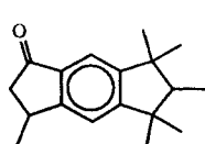
11 strong
