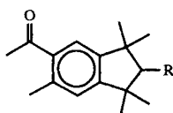
3 R = H, medium
