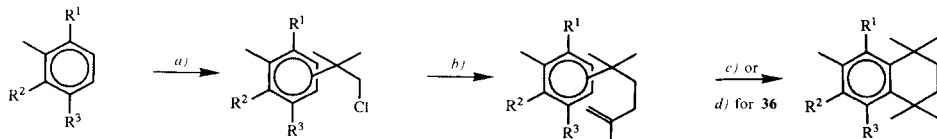
Scheme 3
