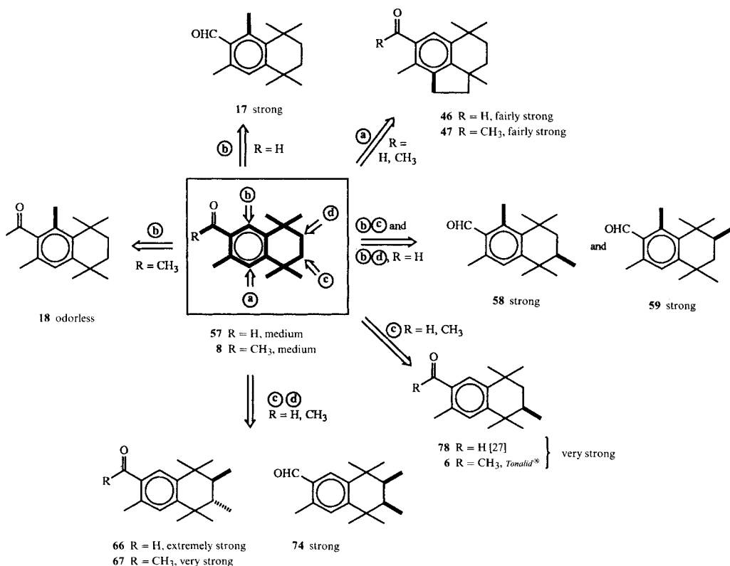
Scheme 10
