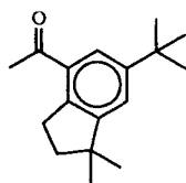
2 strong ( Celestolide a) )
