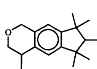
14 strong ( Galaxolide
