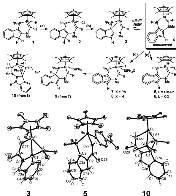
Figure 1. Reagents: (a) CH 2 Cl 2 ; (b) NaN(SiMe 3 ) 2 ; (c) DMAP (DMAP = 4-dimethylaminopyridine, for 5 ) or CO (for 6 ); (d) Ph 3 SiH (for 7 ) or Ph 2 SiH 2 (for 8 ). ORTEP diagrams shown with 50% ellipsoids; selected C and H atoms have been omitted for clarity. Bond lengths (Å) for 3 : Ru–P 2.2158(5); Ru–C1 2.250(2); Ru–C27 1.941(2); P–C1 1.805(2); N–C2 1.397(2); N–C27 1.346(2). Bond lengths (Å) for 5 : Ru–P 2.3011(9); Ru–C27 1.949(3); Ru···C3 (shortest Ru–indenide distance) 3.403; P–C3 1.779(3); N–C2 1.425(4); N–C27 1.329(4). Bond lengths (Å) for 10 : Ru–P 2.295(2); Ru–Si 2.391(2); Ru–H 1.48(9); Ru–C27 2.169(8); P–C1 1.889(7); Si–C1 1.958(8); Si–H 1.90(8); N–C2 1.37(1); N–C27 1.47(1).
