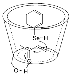
Fig. 2. Supramolecular addition of benzeneselenol to conjugated alkenes within β-CD
