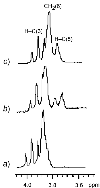
Fig. 1. 1 H-NMR Spectra (D 2 O, 25°) of a) β-CD, b) the β-CD/benzeneselenol complex, and c) the reaction mixture of the β-CD/benzeneselenol complex and methyl vinyl ketone after 15 min
