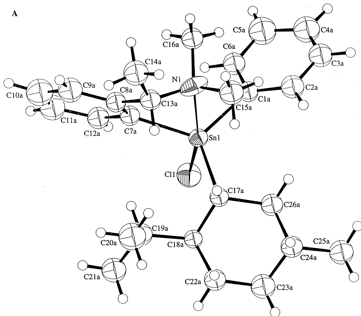
Fig. 2. Molecular structures and atomic numbering scheme for (A) molecule a, and (B) molecule c, of \text{MenPhL}^*\text{SnCl} ( 3 ); the numbering scheme for molecule b follows that of molecule a.
