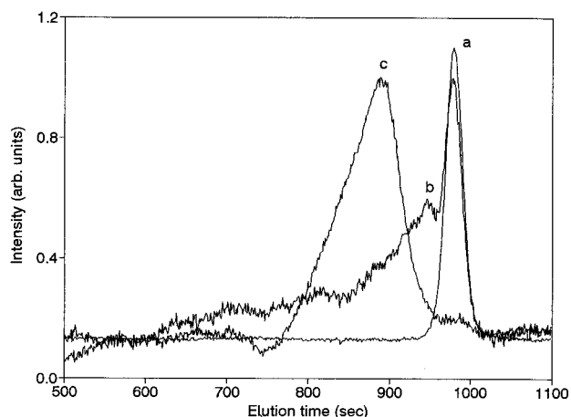
Figure 7. Gel permeation chromatograms for 14βGP (a) before and (b) after 4 h irradiation in the solid I phase at 25–35 °C, and (c) after 2 h irradiation in the melt (“isotropic”) phase at 130 °C. The shape of the peak for the 14βGP product after irradiation of a 10^{-5} M N_2 -saturated benzene solution is virtually the same as in (a).
