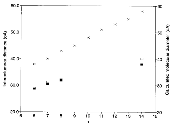
Figure 3. Intercolumnar distances from powder X-ray diffraction data of the mesophases ( \alpha series: ■; \beta series: □) and calculated molecular diameters (Å, from MM + , X) versus alkyl chain length ( n ).
