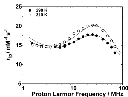
Fig. 2 1/T_1 ^1\text{H} NMRD profiles of \text{Gd}_2\text{L2} at 298 (●) and 310 K (○). The solid lines are calculated with the parameters of Table 2.
