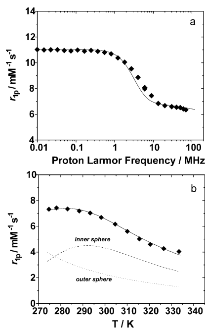
Fig. 1 a) 1/T_1 ^1\text{H} NMRD profile for \text{Gd}_2\text{L1} at 298 K and pH = 7.2. The solid line represents the best-fit to the experimental points (see Table 2). b) Proton relaxivity as a function of temperature for \text{Gd}_2\text{L1} at 20 MHz. The solid line represents the best-fit to the experimental data (Table 2), whereas the dotted and dashed lines represent the calculated outer- and inner-sphere contributions to the relaxivity.
