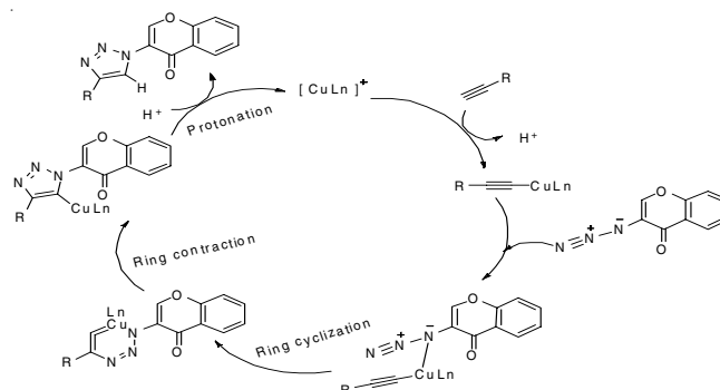
Fig. 1. Plausible mechanism of 1,3-dipolar cycloaddition of 5a to alkynes
