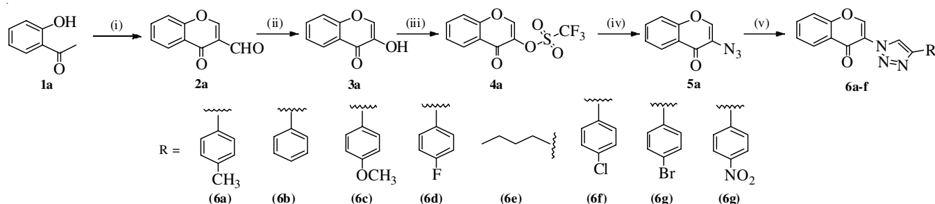
Scheme-I: Synthesis of chromone-1,2,3-triazole hybrids ( 6a-h ); Reaction conditions: (i) POCl 3 in DMF, room temperature, 24 h, yield 75-80%. (ii) m -CPBA, DCM, 40 °C reflux, 24 h, yield 70%. (iii) Trifluoro methane sulfonic anhydride, triethylamine in DCM, 0 °C, room temperature, 3 h, yield 70-75%. (iv) NaN 3 , DMF, 90 °C, 3 h, yield 60%. (v) CuI, alkyl/aryl acetylenes, DMSO, 60 °C, 1 h, yield 80%
