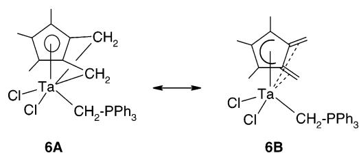
Scheme 1. Two Resonance Forms of Complex 6
