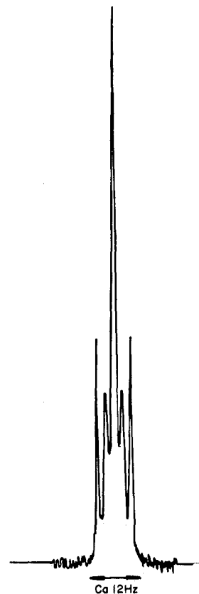
Figure 1.—Methyl resonance pattern observed in the nmr spectra of \{Rh[P(OCH_3)_2C_6H_5]_4\}PF_6 and \{Rh[POCH_3(C_6H_5)_2]_4\}PF_6 .
