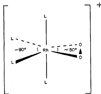
Figure 2.—Proposed structure for the cations RhL_4O_2^+ .
