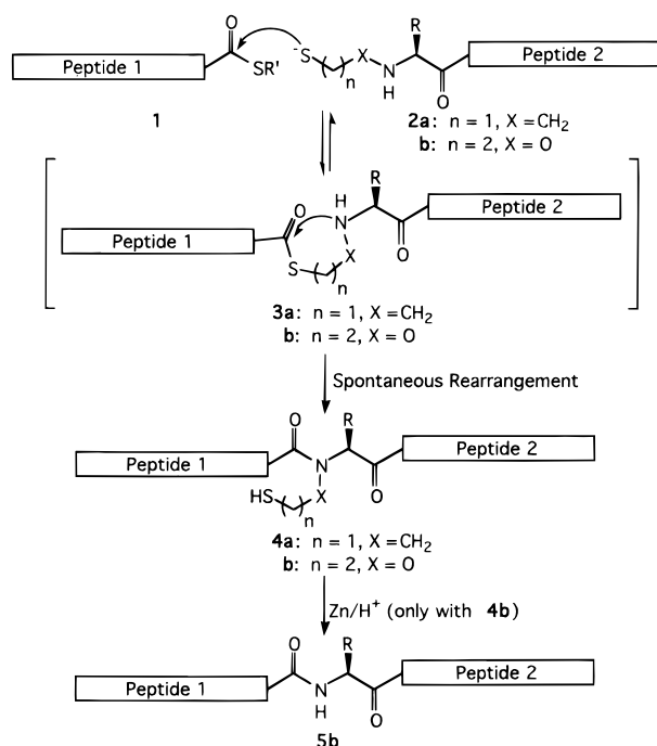
Scheme 1. Generalized Native Chemical Ligation of Unprotected Peptide Segments
