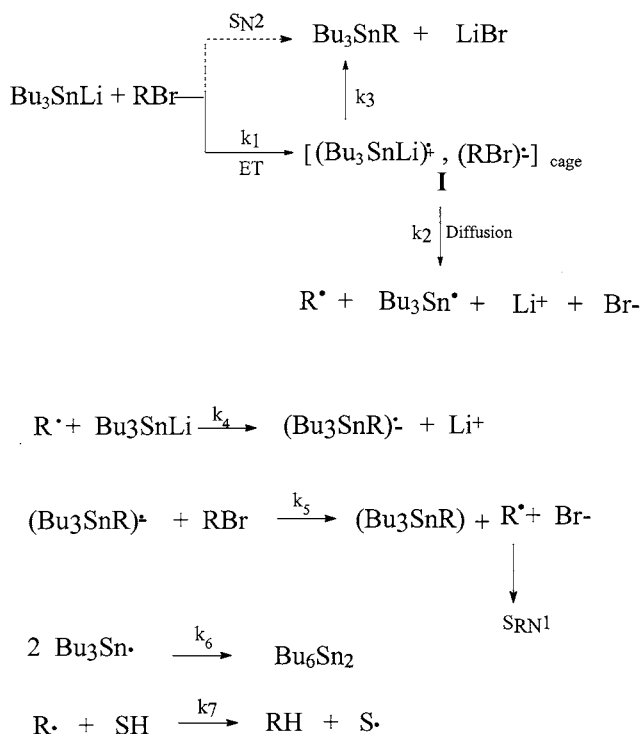
Scheme 1. The reaction scheme of (tributyltin)lithium with alkyl and aryl bromides.
