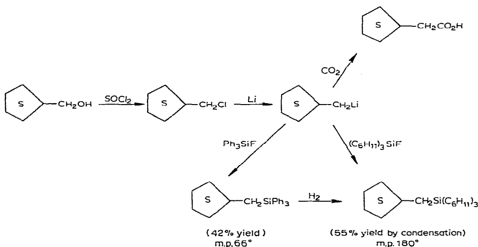
Fig. 1. Synthesis path for tricyclohexyl(cyclopentylmethyl)silane.
